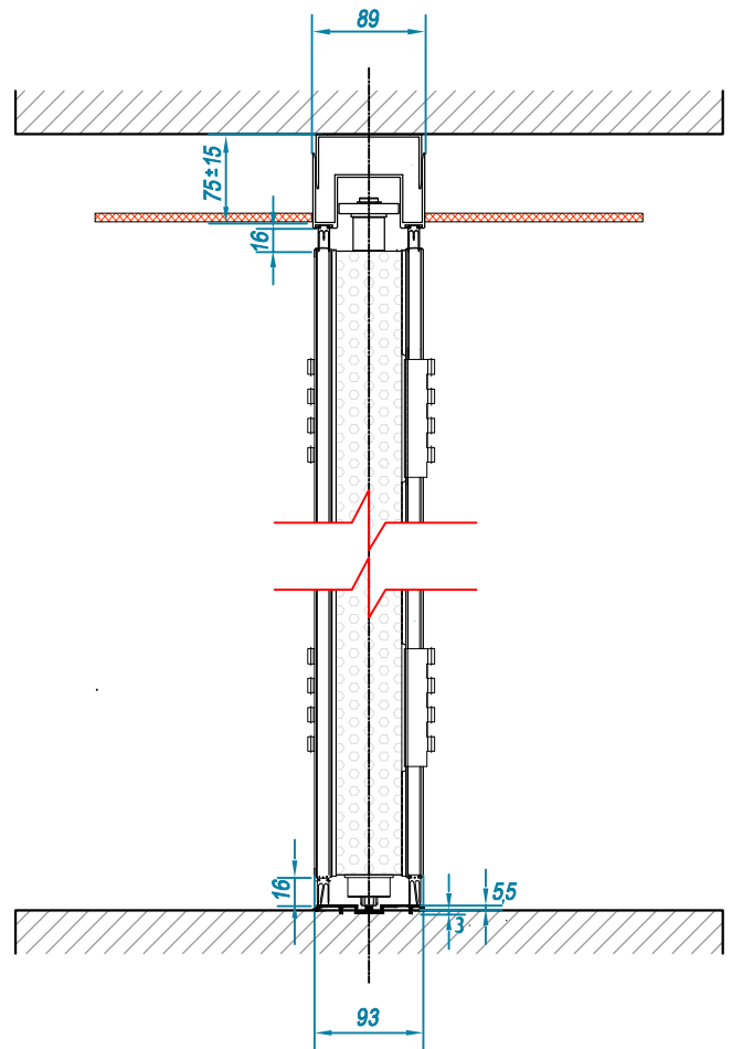
Top-bottom mount
